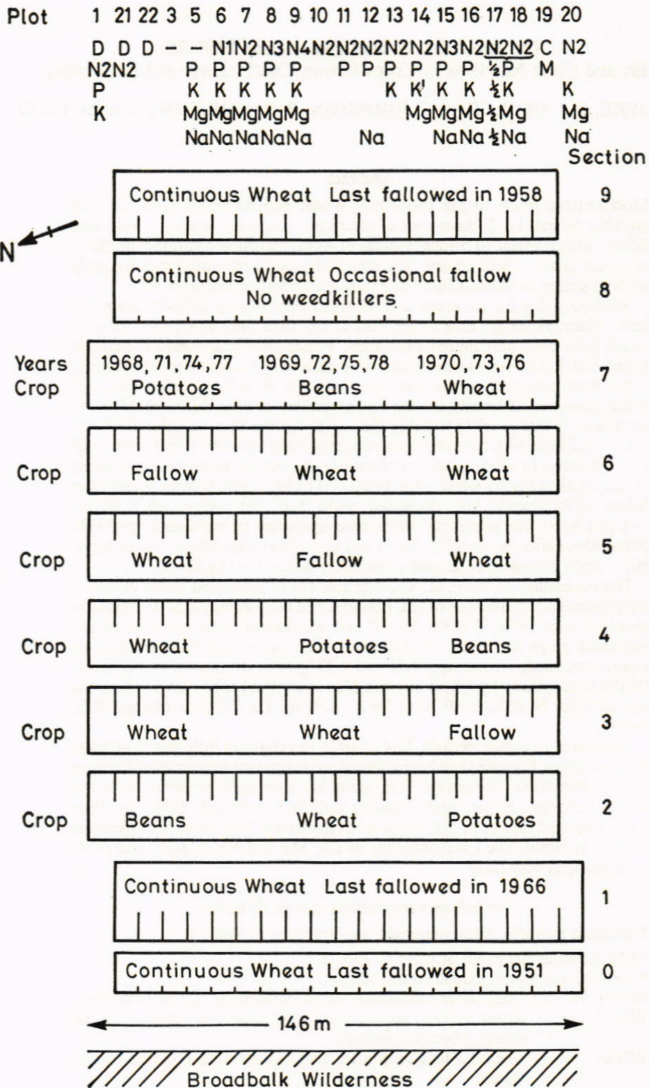
FIG. 1. Plan of the Broadbalk Wheat experiment showing sections, plots, manuring and crop ping from 1968. For details of treatments see Table 1.
