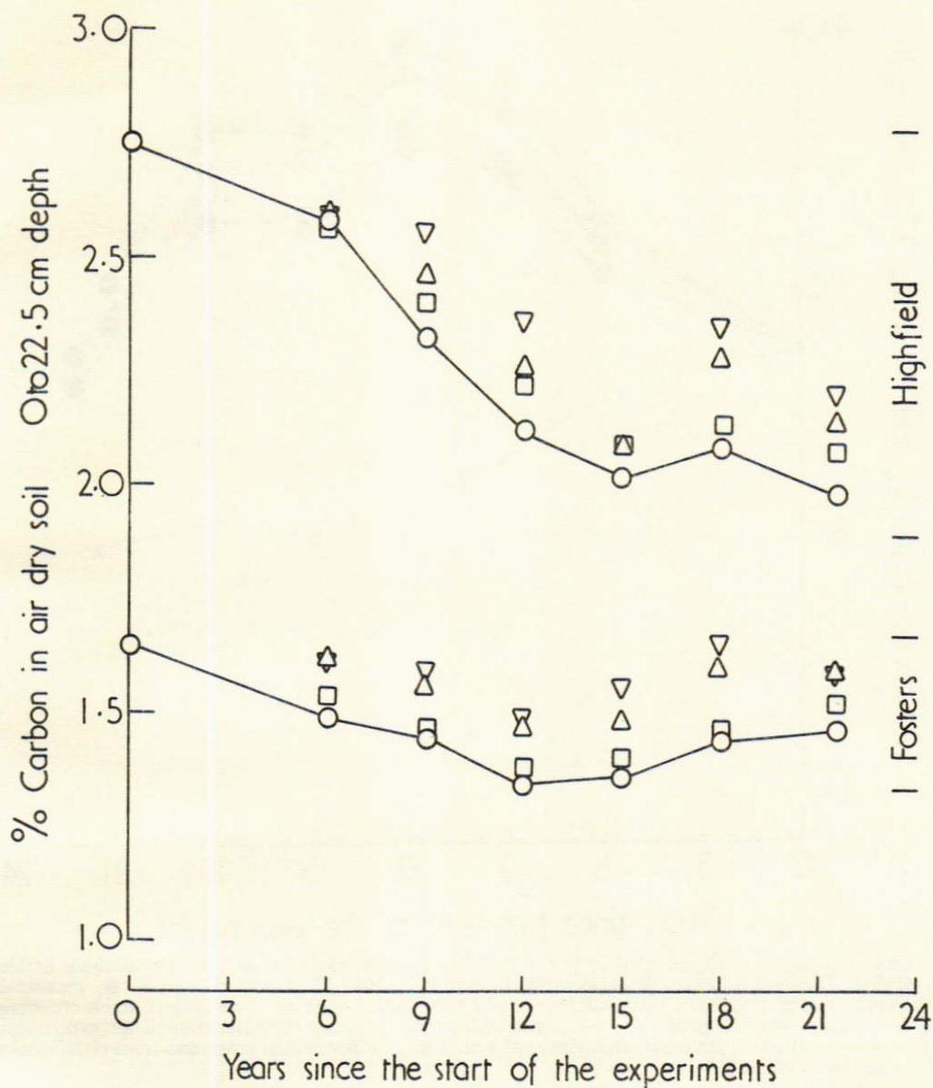
FIG. 1. Changes in organic carbon in soil caused by ley and arable cropping systems. Rothamsted Ley-Arable experiments, 1949-72. Continuous arable cropping, ○; ley-arable cropping systems, lucerne, □; cut grass/ley-with-N, △; grazed ley/ley-with-clover, ▽. (Results are means from eight blocks for each experiment for 6, 9, 12 and 21/22 years and from four blocks for 15 and 18 years.)
