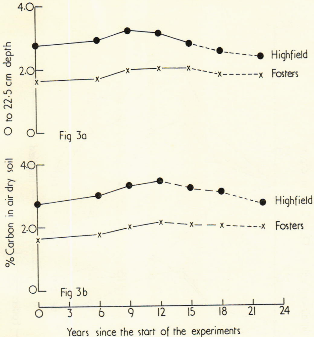
FIG. 3. Changes in organic carbon in soil under the reseeded grass. Rothamsted Ley-Arable experiments, 1949-72. Highfield, ●; Fosters, ×. FIG. 3a. Grass grazed for 15 years then ploughed and arable crops grown continuously for 6 to 7 years. Grass grazed —; all-arable cropping, - - - - -. FIG. 3b. Grass grazed for 12 years then cut at silage stage for six years, then ploughed and arable crops grown continuously for three to four years. Grass grazed, —; grass cut — —; all arable cropping, - - - - -. (Results are means from all 12 blocks in both experiments.)
