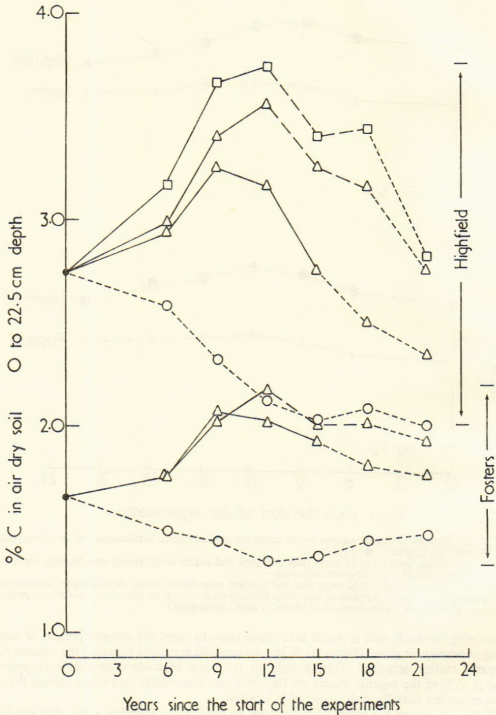
FIG. 4. Changes in organic carbon in soil under continuous arable cropping, ○; reseeded grass, △ and permanent grass, □. Rothamsted Ley-Arable experiments, 1949-72. Grass grazed —, grass cut at silage stage —, arable crops grown continuously -----. (Results are means from blocks 5 to 12 inclusive in both experiments.)
